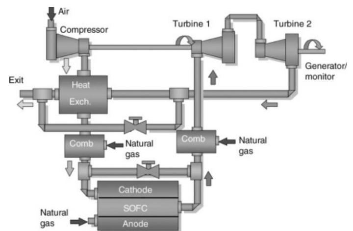
Figure 8. Pressure HTFC and gas turbine hybrid system [43]
