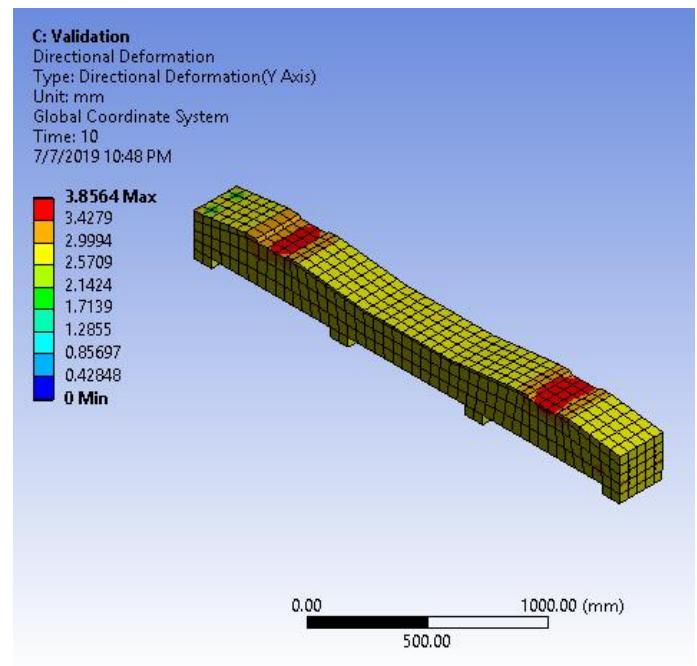
Figure 1. Deformation at 237.5 kN
